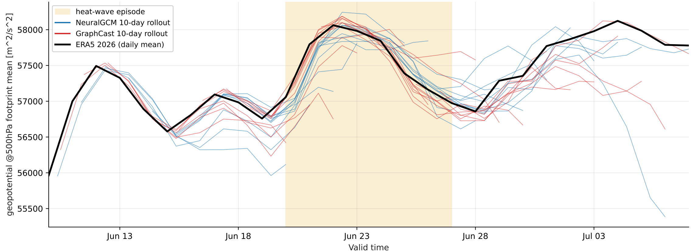
Europe heat-wave 2026-06-20..2026-06-27 — footprint-mean geopotential @ 500 hPa (cortex, > p99)
