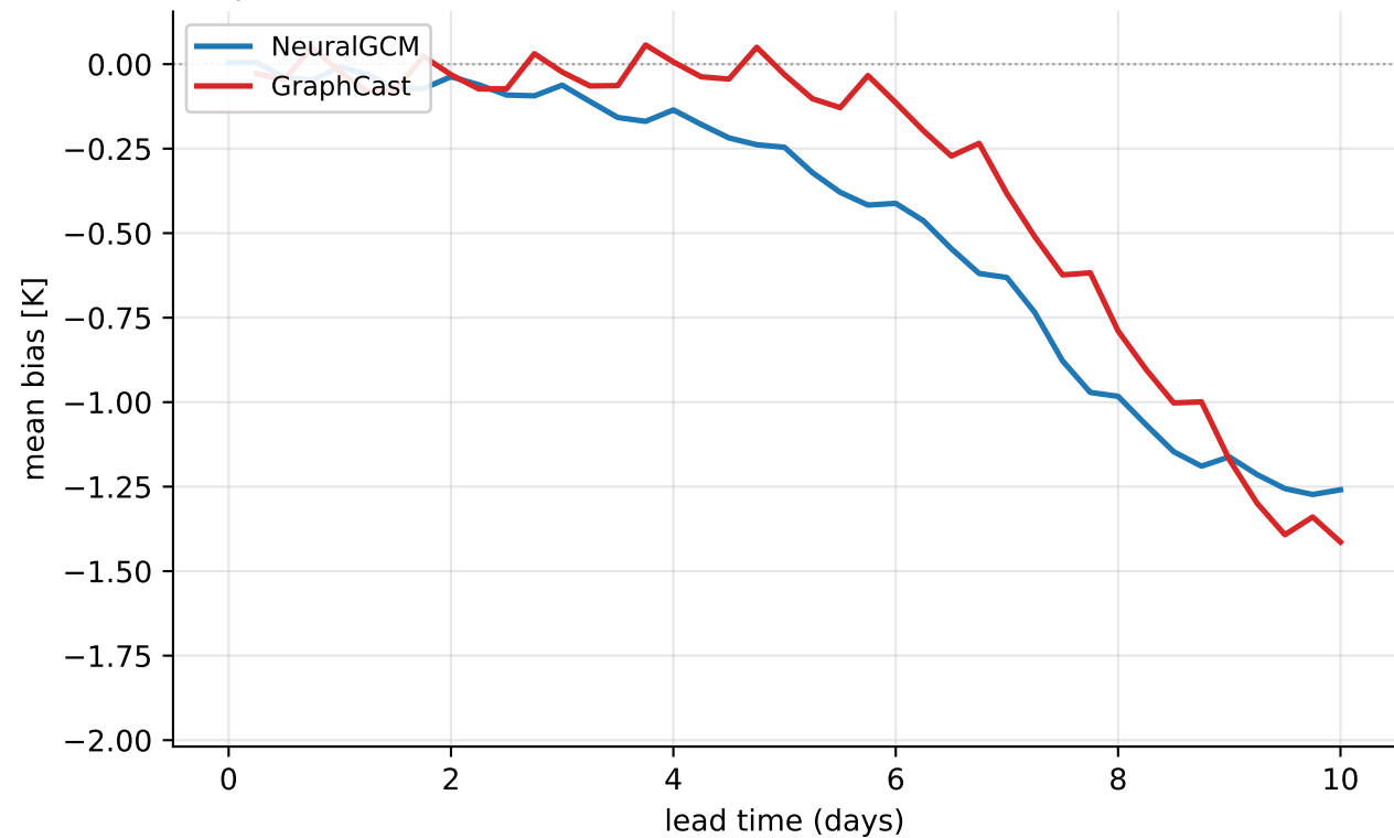
temperature@850 hPa — mean bias over the 10 2023 mixture heat waves (10 events, > p99)
