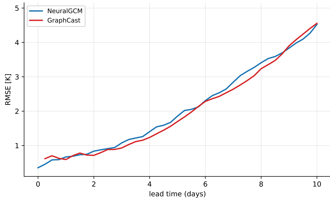
temperature@850 hPa — mean RMSE over the 10 2023 mixture heat waves (10 events, > p99)
