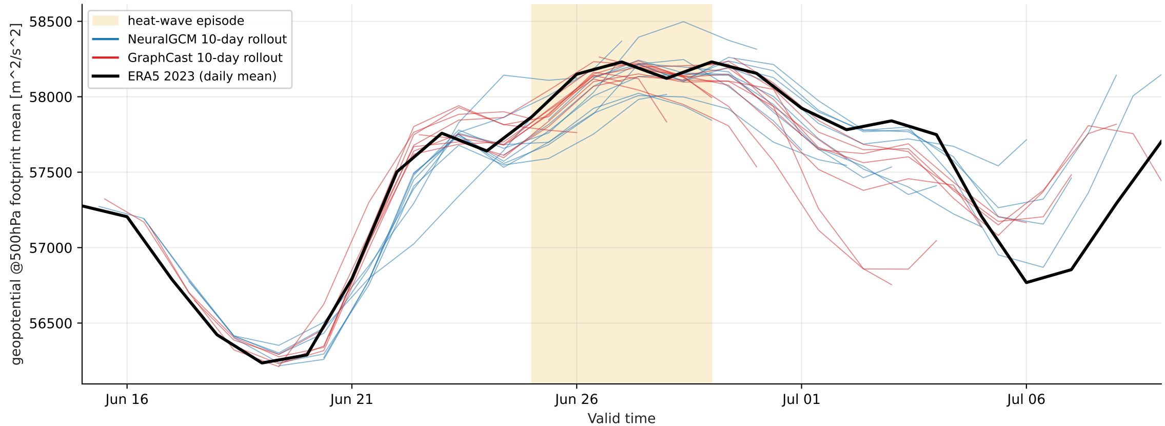
Europe heat-wave 2023-06-25..2023-06-29 — footprint-mean geopotential @ 500 hPa (mixture, > p99)
