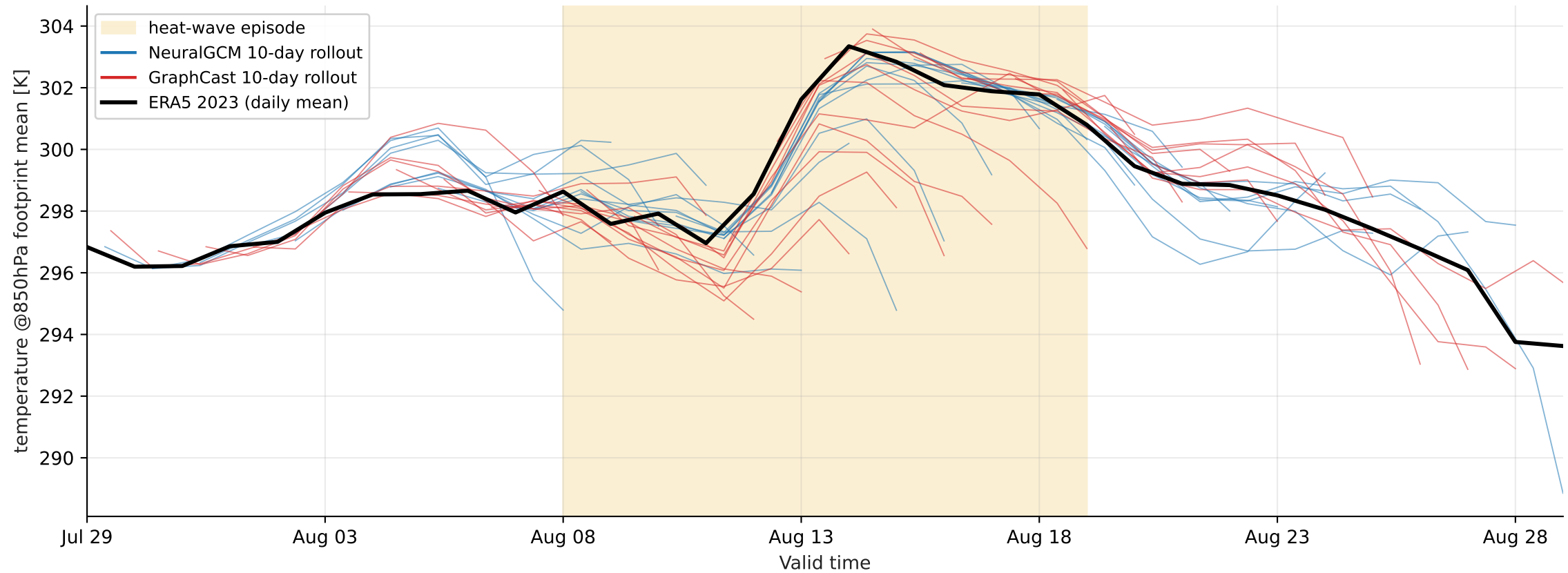
Europe heat-wave 2023-08-08..2023-08-19 — footprint-mean temperature @ 850 hPa (mixture, > p99)
