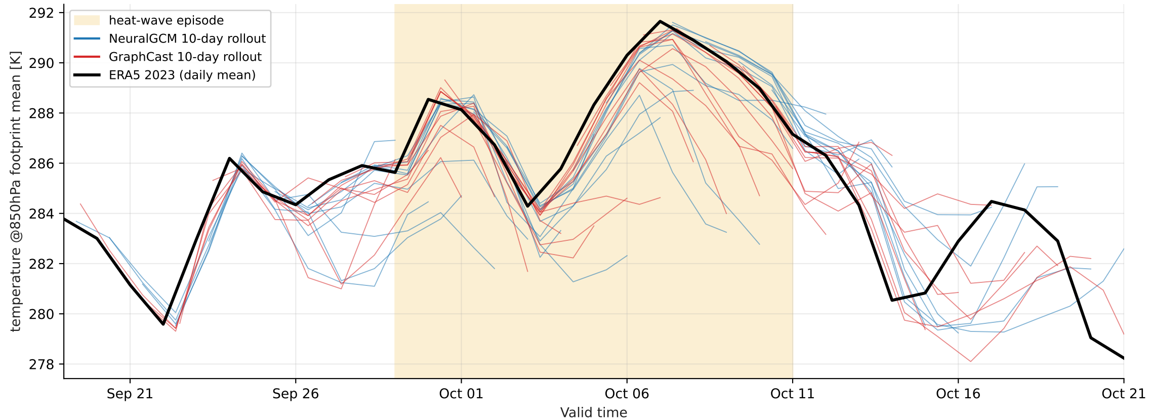
Europe heat-wave 2023-09-29..2023-10-11 — footprint-mean temperature @ 850 hPa (mixture, > p99)
