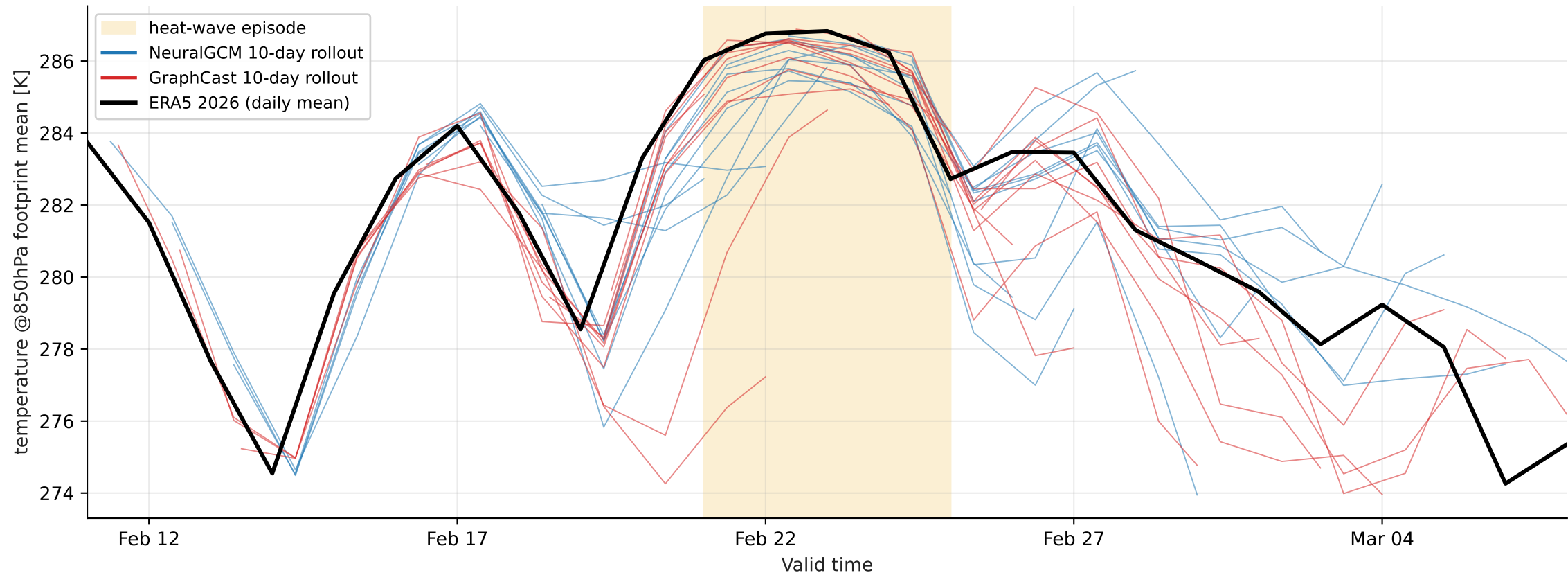
Europe heat-wave 2026-02-21..2026-02-25 — footprint-mean temperature @ 850 hPa (mixture, > p99)
