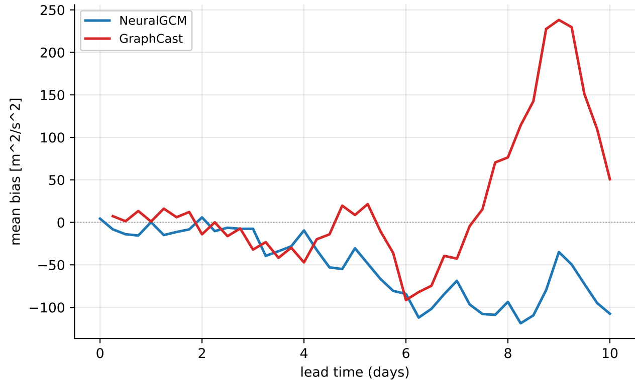
Europe heat-wave 2026-05-22..2026-06-01 — footprint geopotential@500 hPa (mean of 21 rollouts)
