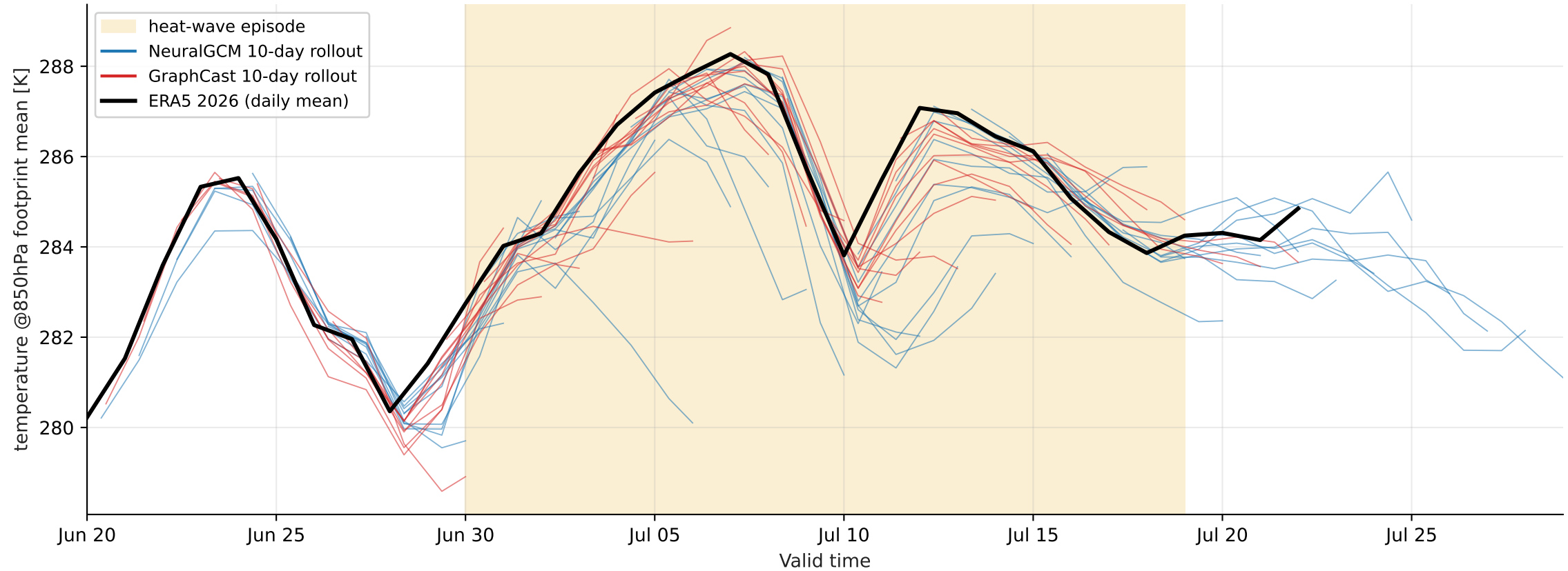
Europe heat-wave 2026-06-30..2026-07-19 — footprint-mean temperature @ 850 hPa (mixture, > p99)
