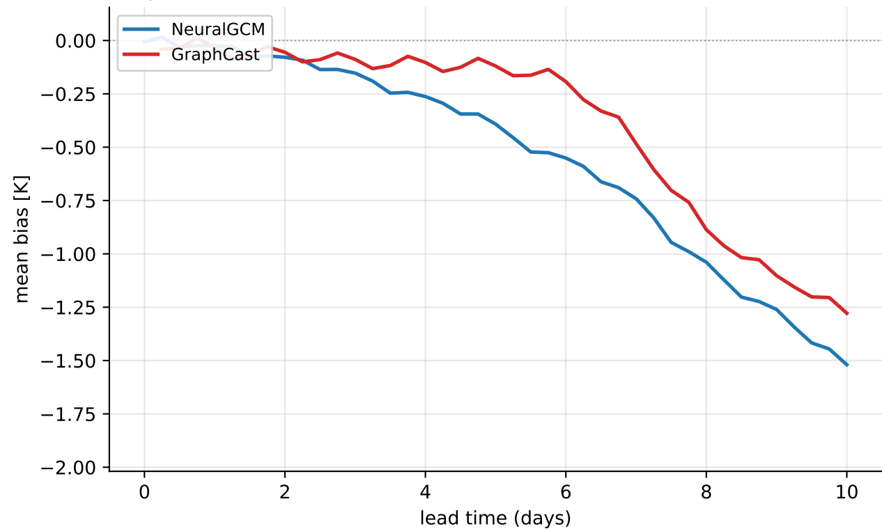
temperature@850 hPa — mean bias over all mixture heat waves (16 events, > p99)
