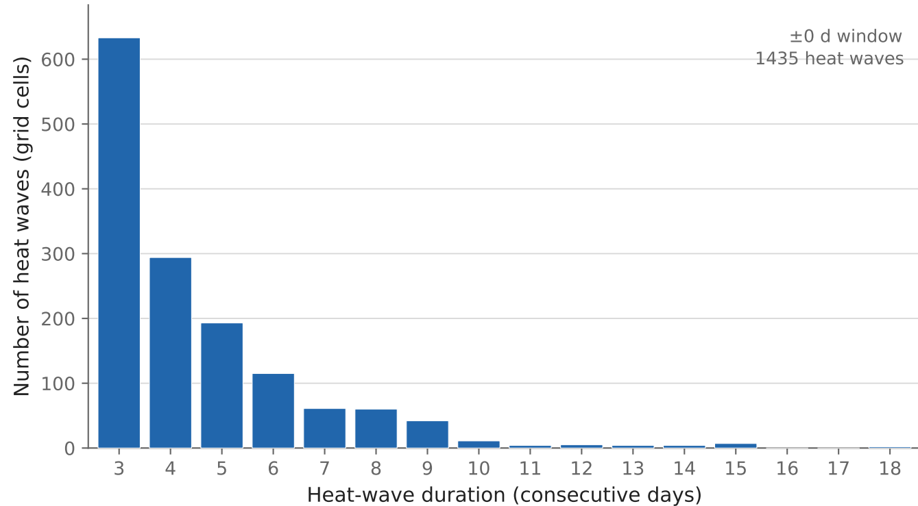
Europe — 2023 heat-wave duration spectrum — event count 95th-pctile T_{850} (00 UTC), 1991-2020 reference, \pm 0 -day window, \geq 3 -day spells, 2.8^\circ grid
