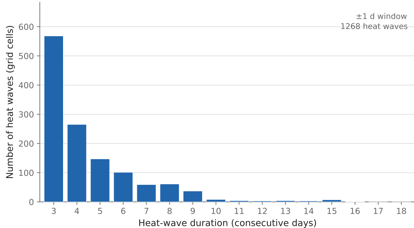
Europe — 2023 heat-wave duration spectrum — event count 95th-pctile T_{850} (00 UTC), 1991-2020 reference, \pm 1 -day window, \geq 3 -day spells, 2.8^\circ grid
