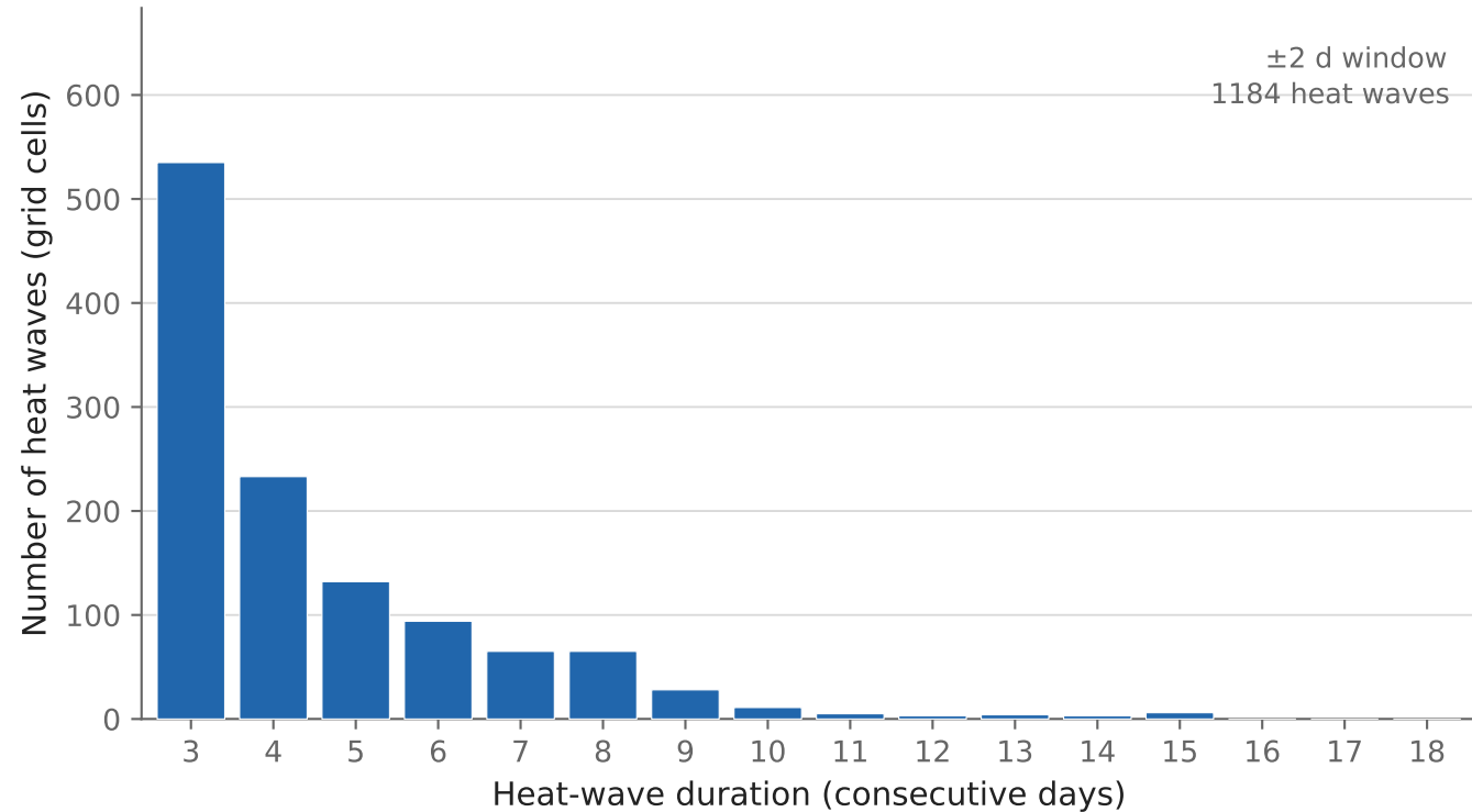
Europe — 2023 heat-wave duration spectrum — event count 95th-pctile T_{850} (00 UTC), 1991-2020 reference, \pm 2 -day window, \geq 3 -day spells, 2.8^\circ grid
