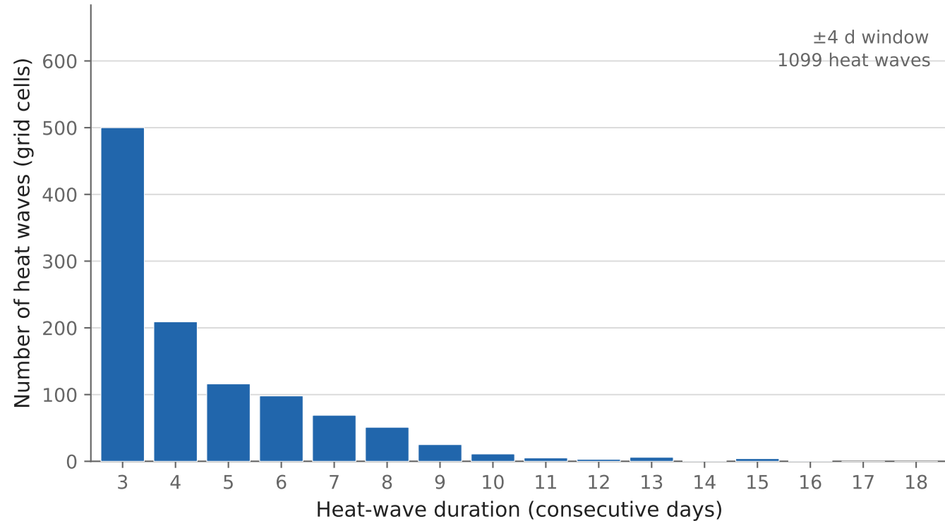
Europe — 2023 heat-wave duration spectrum — event count 95th-pctile T_{850} (00 UTC), 1991-2020 reference, \pm 4 -day window, \geq 3 -day spells, 2.8^\circ grid
