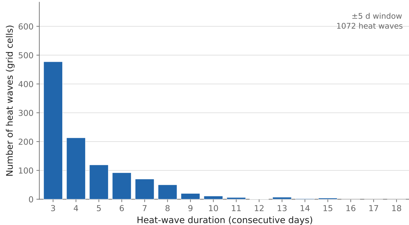
Europe — 2023 heat-wave duration spectrum — event count 95th-pctile T_{850} (00 UTC), 1991-2020 reference, \pm 5 -day window, \geq 3 -day spells, 2.8^\circ grid
