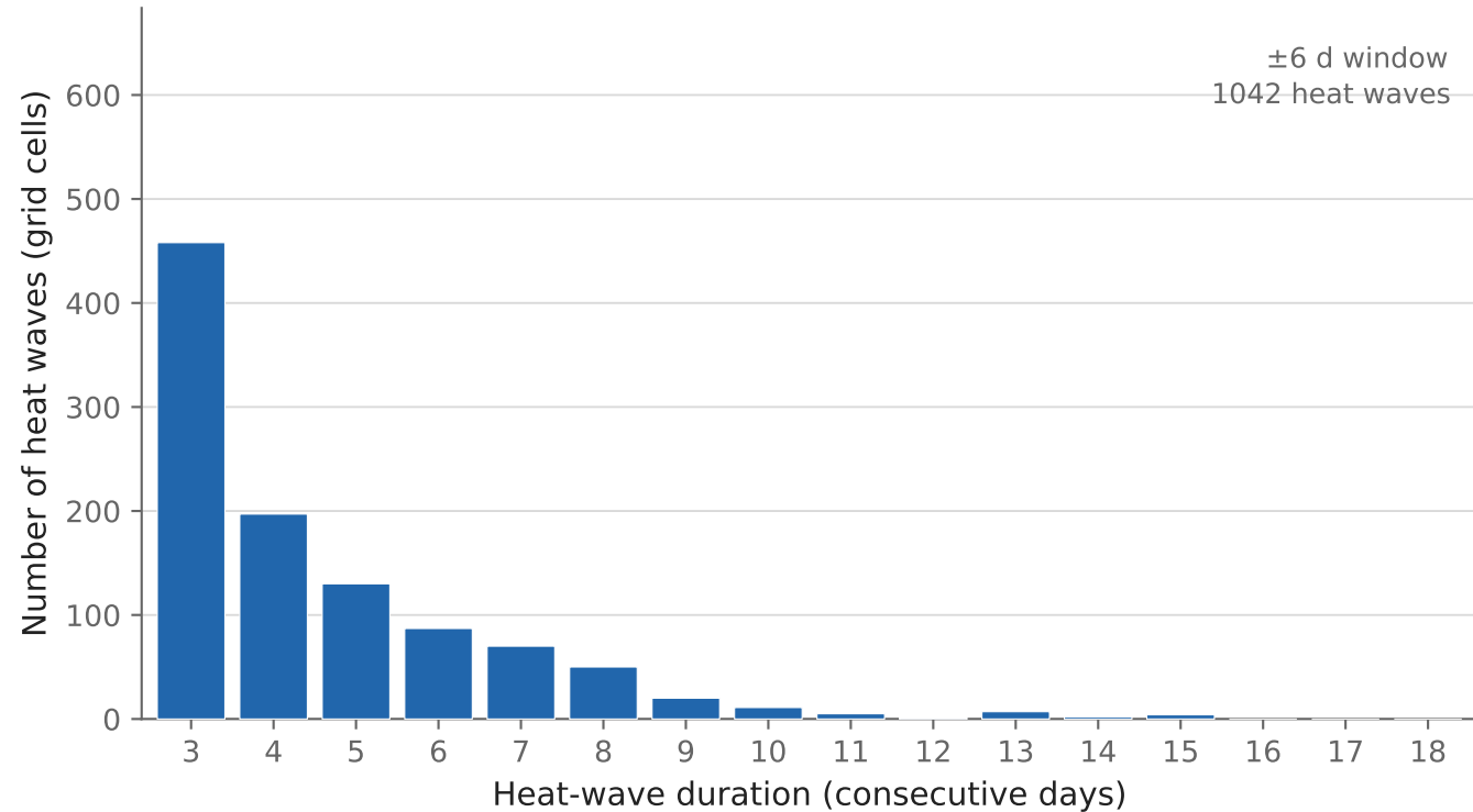
Europe — 2023 heat-wave duration spectrum — event count 95th-pctile T_{850} (00 UTC), 1991-2020 reference, \pm 6 -day window, \geq 3 -day spells, 2.8^\circ grid
