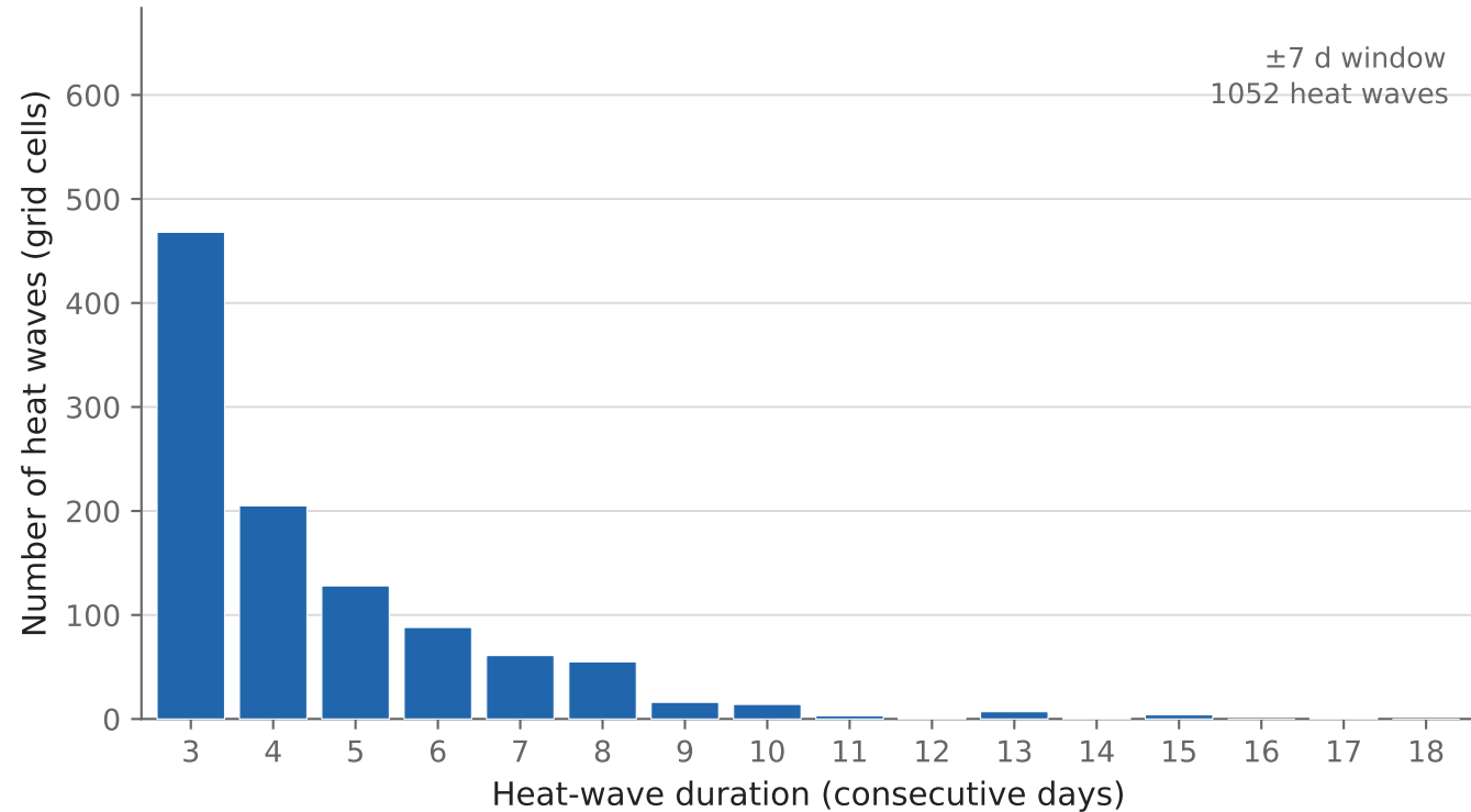
Europe — 2023 heat-wave duration spectrum — event count 95th-pctile T_{850} (00 UTC), 1991-2020 reference, \pm 7 -day window, \geq 3 -day spells, 2.8^\circ grid
