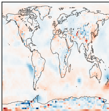
GraphCast
