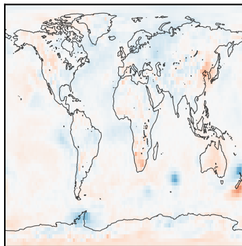
NeuralGCM
