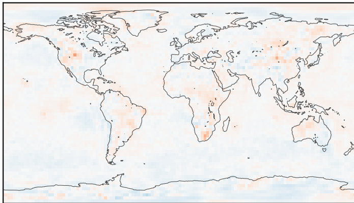
NeuralGCM
