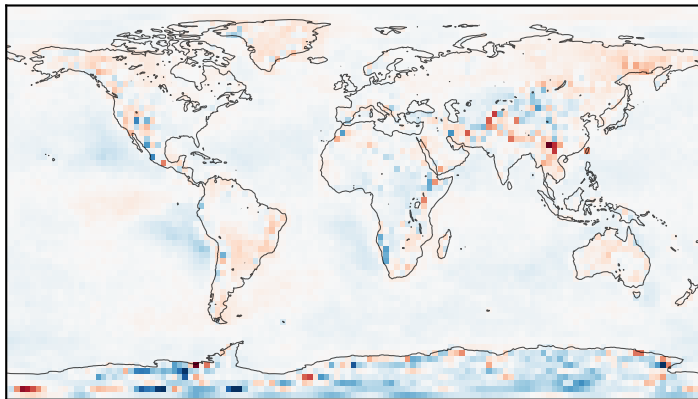
GraphCast
