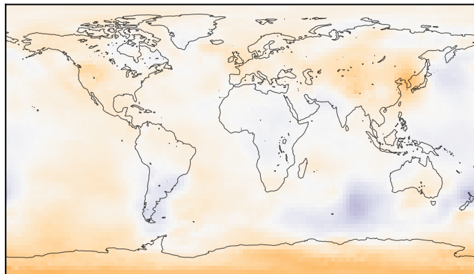
GraphCast
