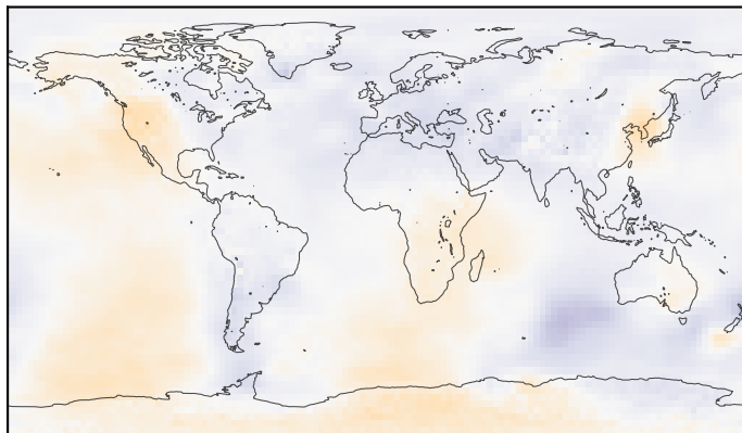
NeuralGCM
