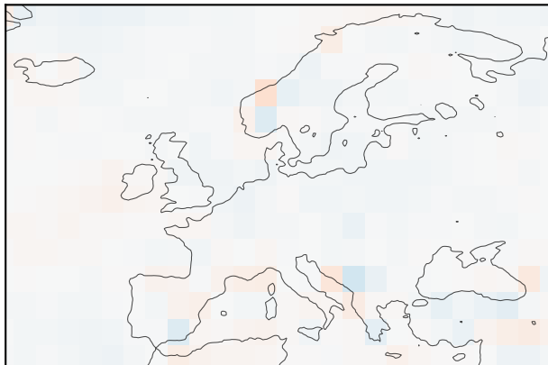
GraphCast
