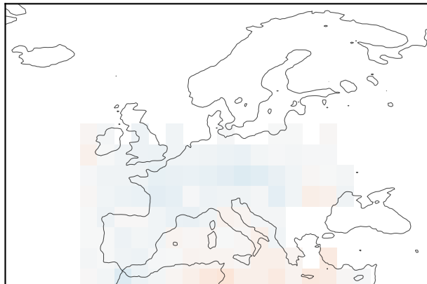
NeuralGCM
