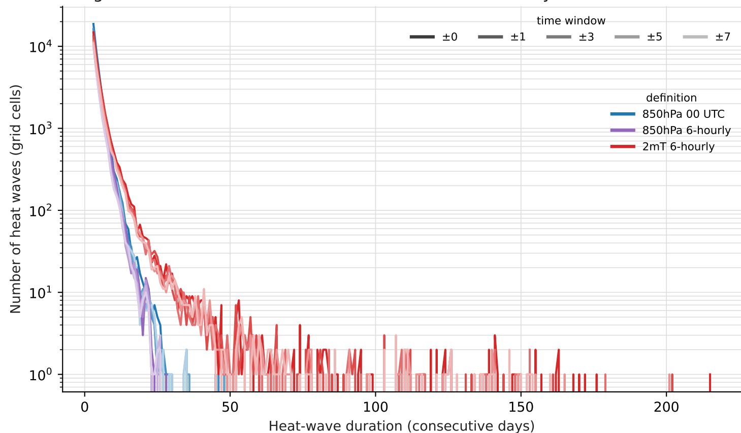
Length of heat wave classification in the world in 2023 by definitions
