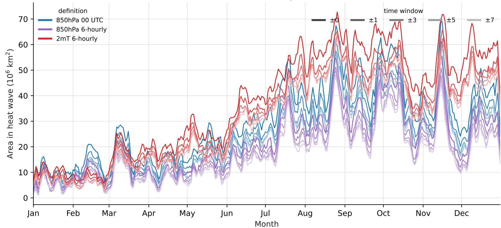
Area classified as heat wave in the world in 2023 by definitions
