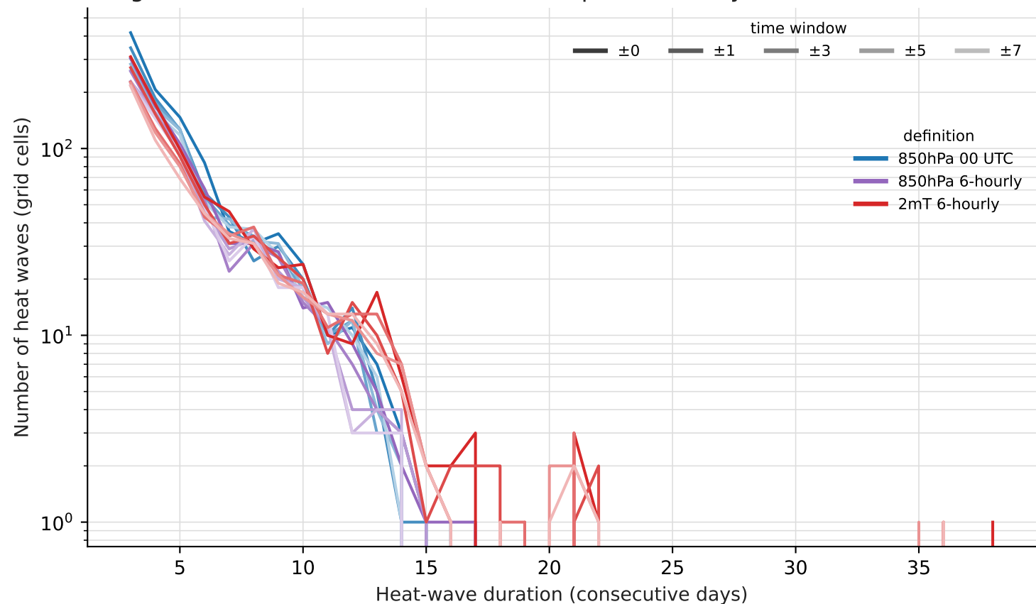
Length of heat wave classification in Europe in 2026 by definitions
