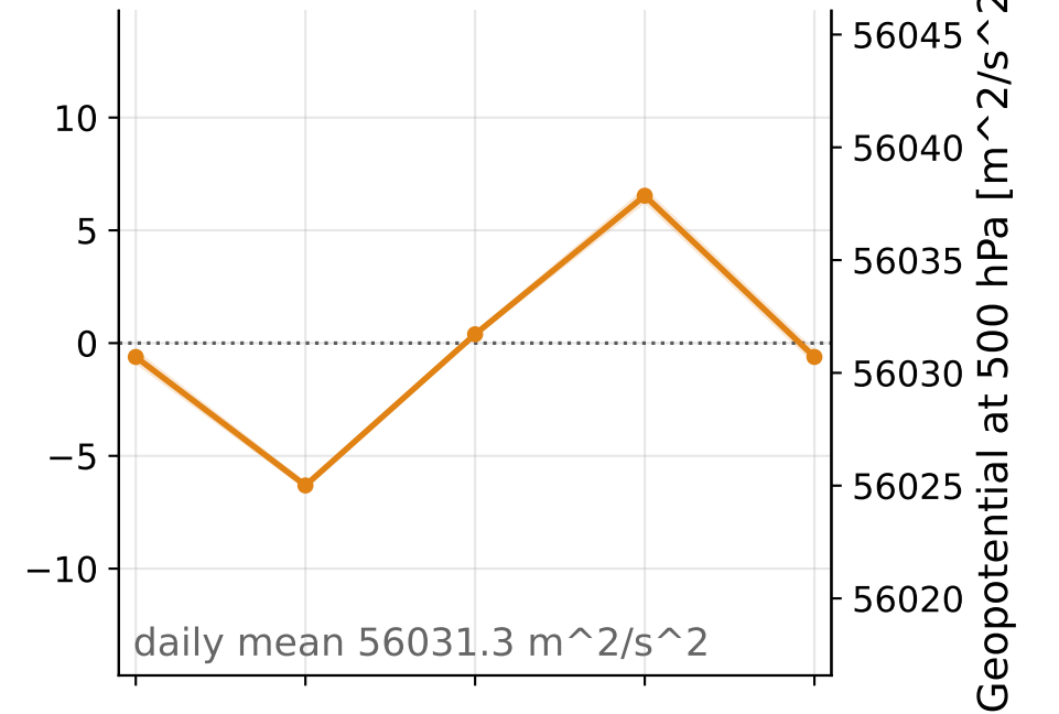
NextGEMS-2049
