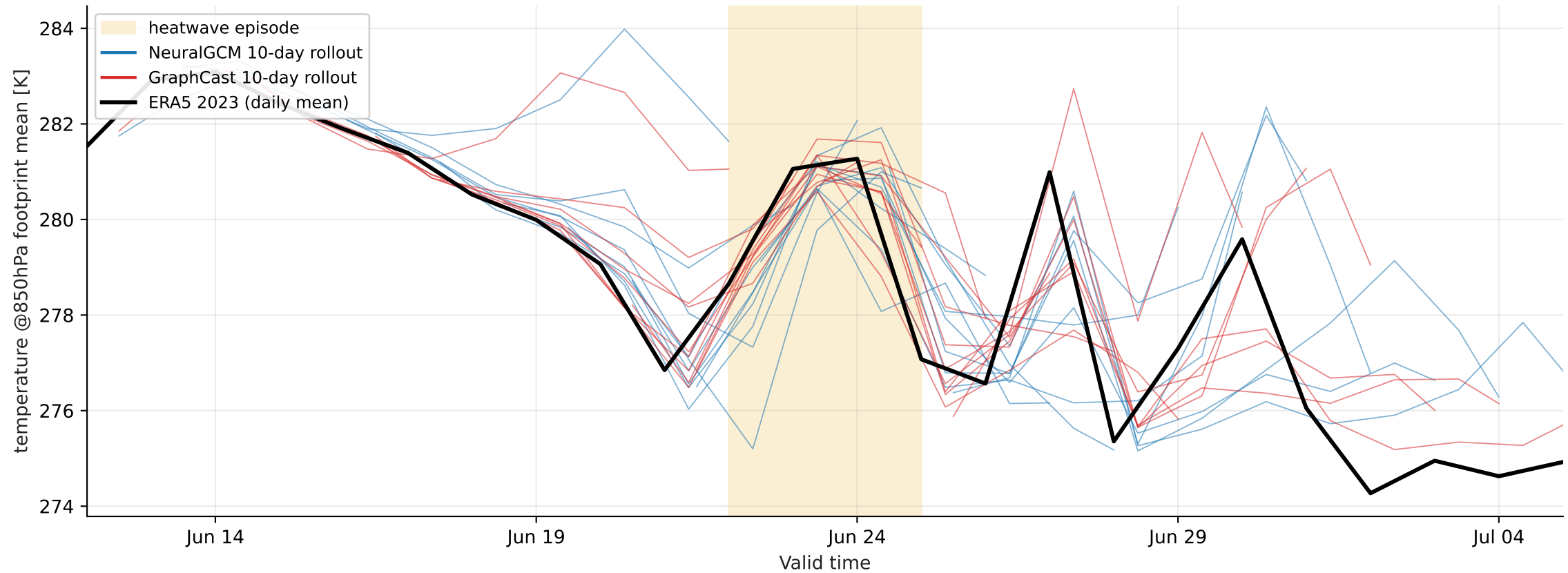
Europe heatwave 2023-06-22..2023-06-25 — footprint-mean temperature @ 850 hPa (cordex, > p99)
