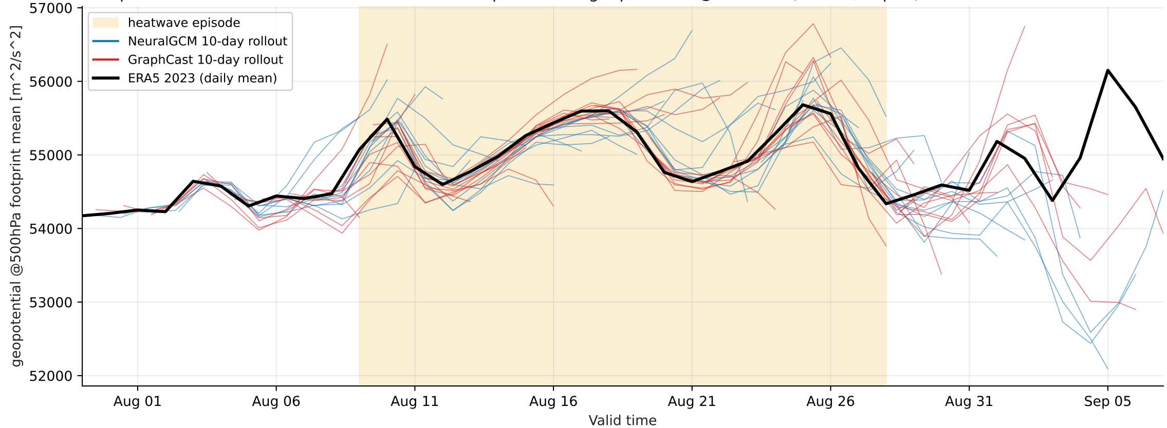
Europe heatwave 2023-08-09..2023-08-28 — footprint-mean geopotential @ 500 hPa (cortex, > p99)
