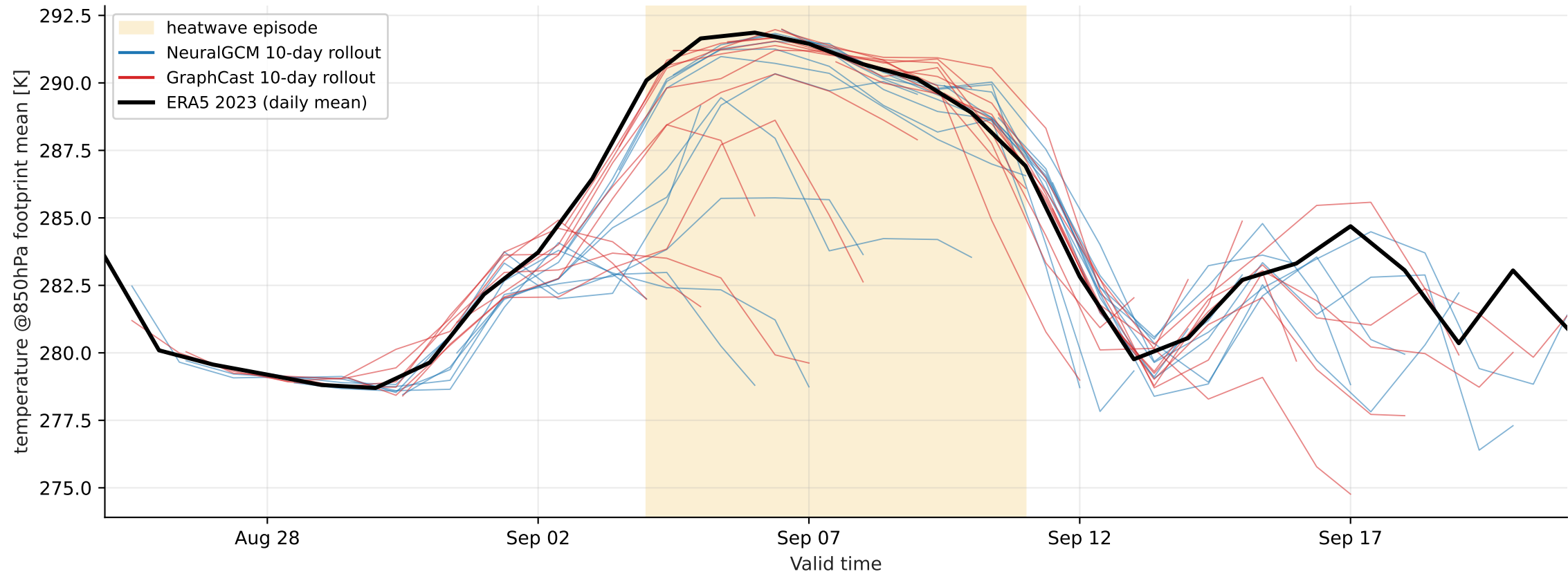
Europe heatwave 2023-09-04..2023-09-11 — footprint-mean temperature @ 850 hPa (cortex, > p99)
