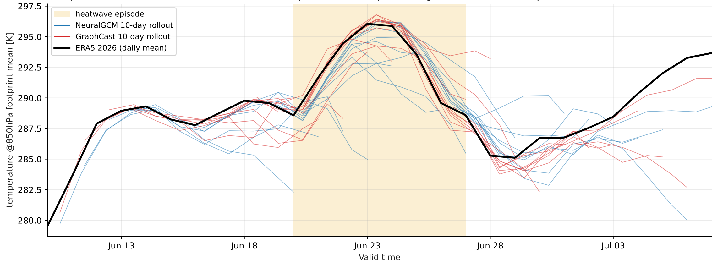
Europe heatwave 2026-06-20..2026-06-27 — footprint-mean temperature @ 850 hPa (cordex, > p99)
