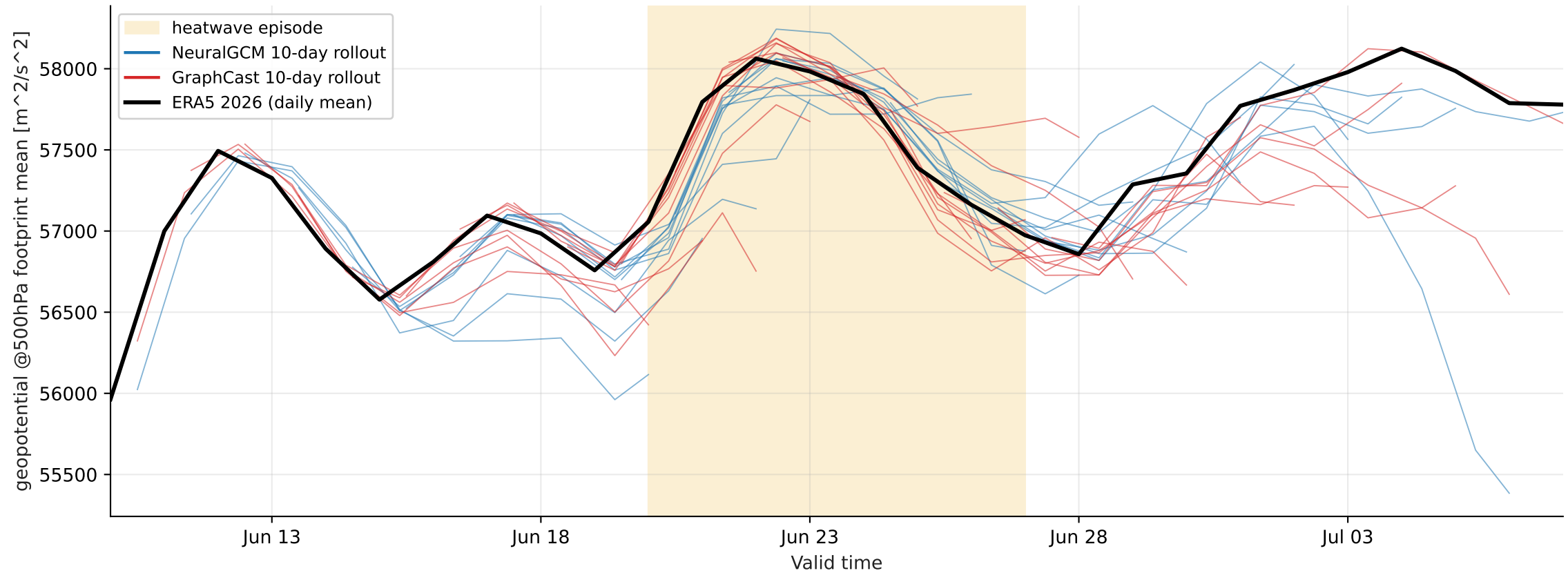
Europe heatwave 2026-06-20..2026-06-27 — footprint-mean geopotential @ 500 hPa (cordex, > p99)
