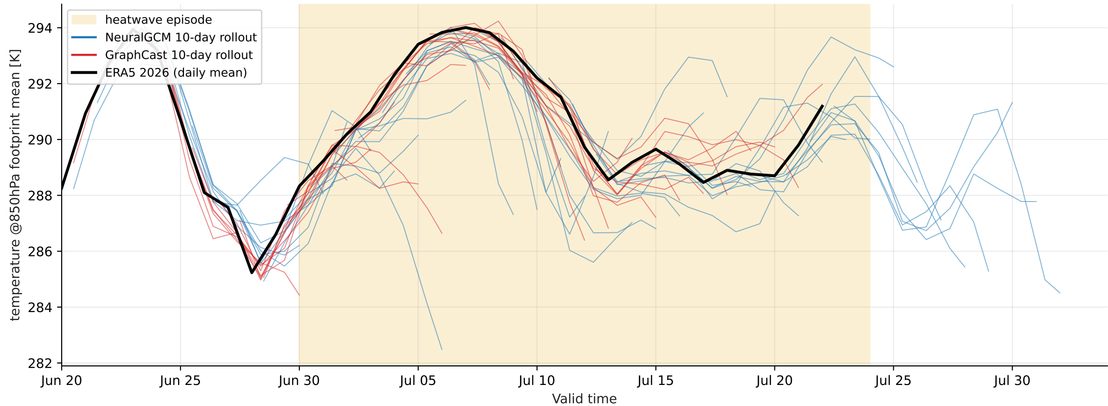
Europe heatwave 2026-06-30..2026-07-24 — footprint-mean temperature @ 850 hPa (cordex, > p99)
