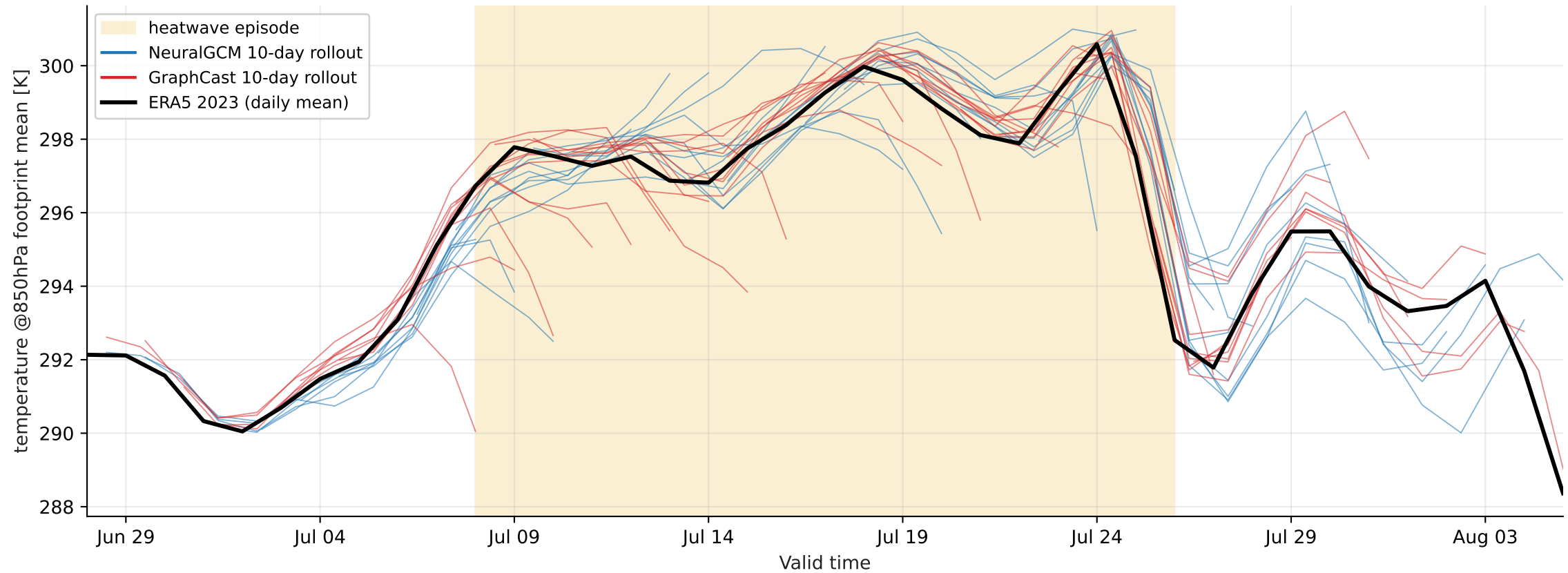
Europe heatwave 2023-07-08..2023-07-26 — footprint-mean temperature @ 850 hPa (mixture, > p99)
