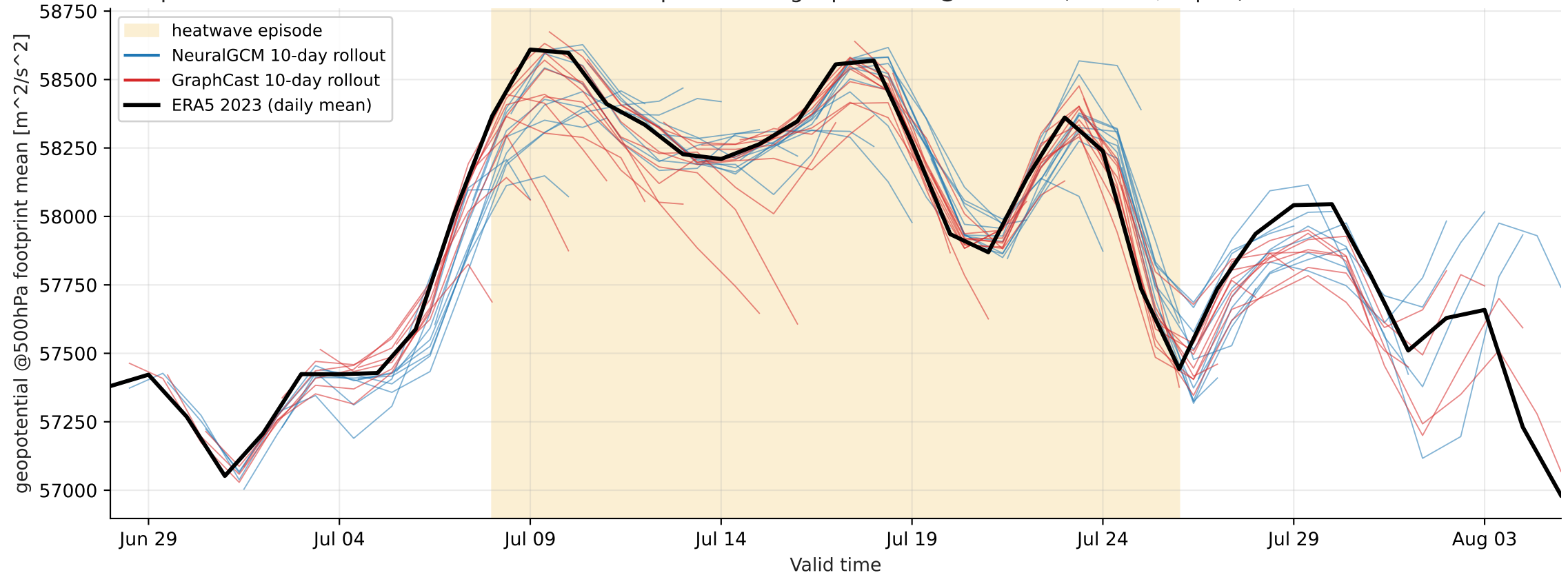
Europe heatwave 2023-07-08..2023-07-26 — footprint-mean geopotential @ 500 hPa (mixture, > p99)
