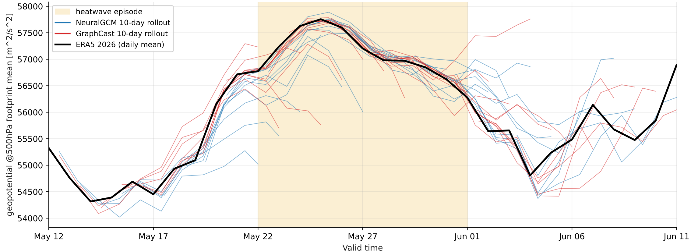
Europe heatwave 2026-05-22..2026-06-01 — footprint-mean geopotential @ 500 hPa (mixture, > p99)
