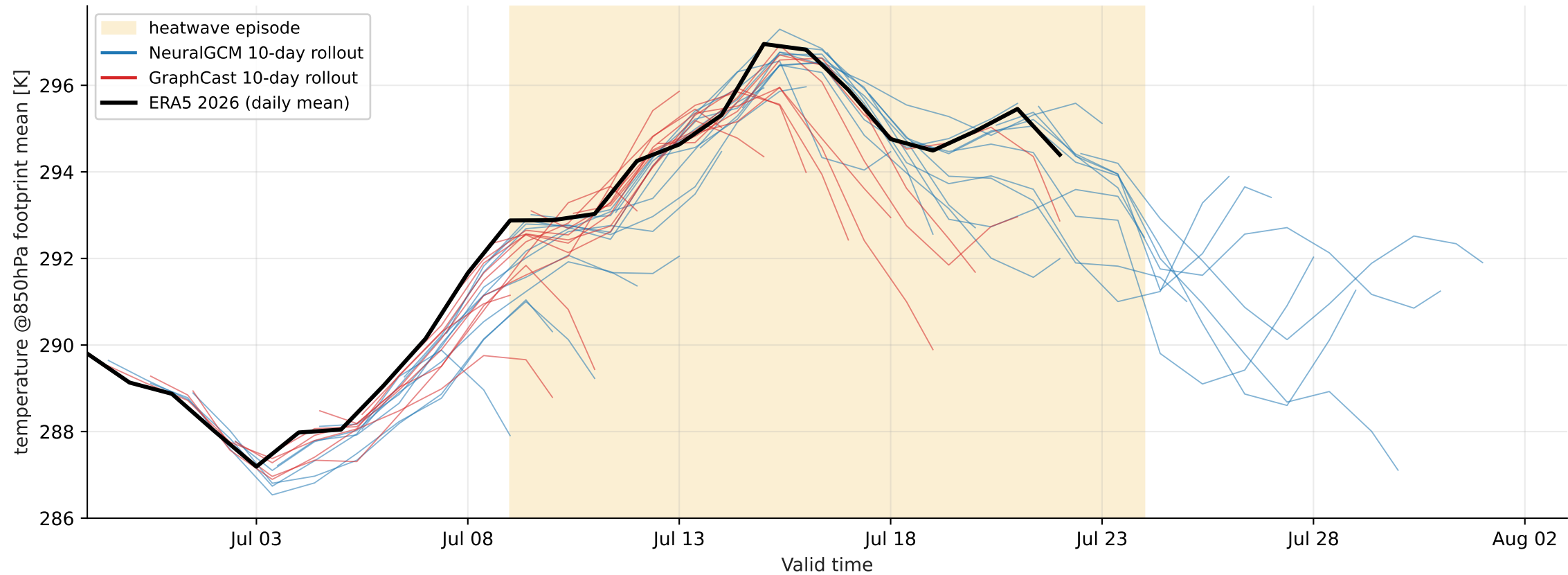
Europe heatwave 2026-07-09..2026-07-24 — footprint-mean temperature @ 850 hPa (mixture, > p99)
