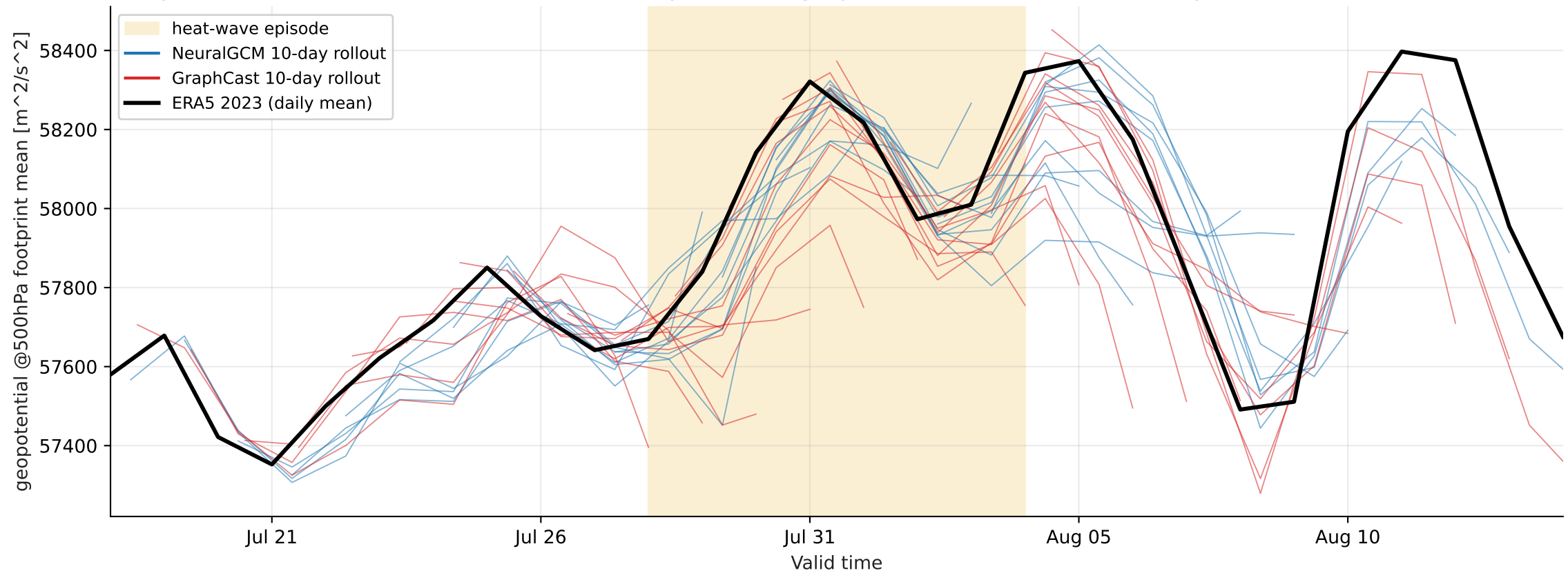
Europe heat-wave 2023-07-28..2023-08-04 — footprint-mean geopotential @ 500 hPa (cordex, > p99)
