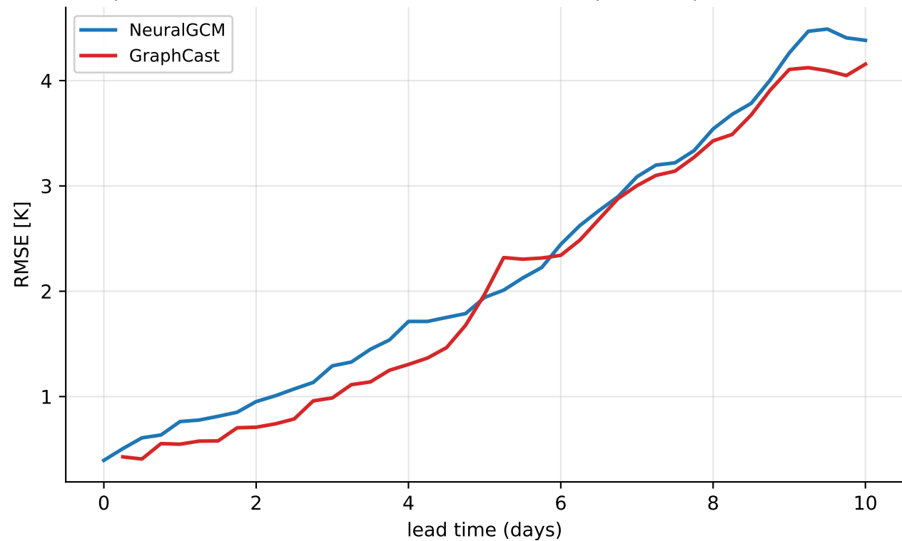
Europe heat-wave 2023-08-09..2023-08-28 — footprint temperature@850 hPa (mean of 30 rollouts)
