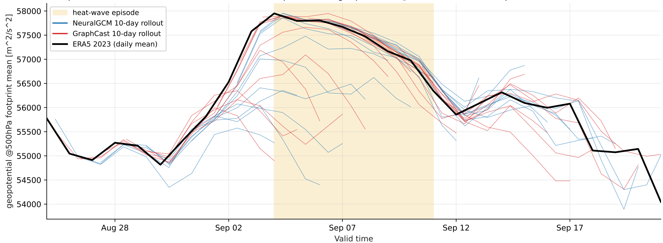
Europe heat-wave 2023-09-04..2023-09-11 — footprint-mean geopotential @ 500 hPa (cordex, > p99)
