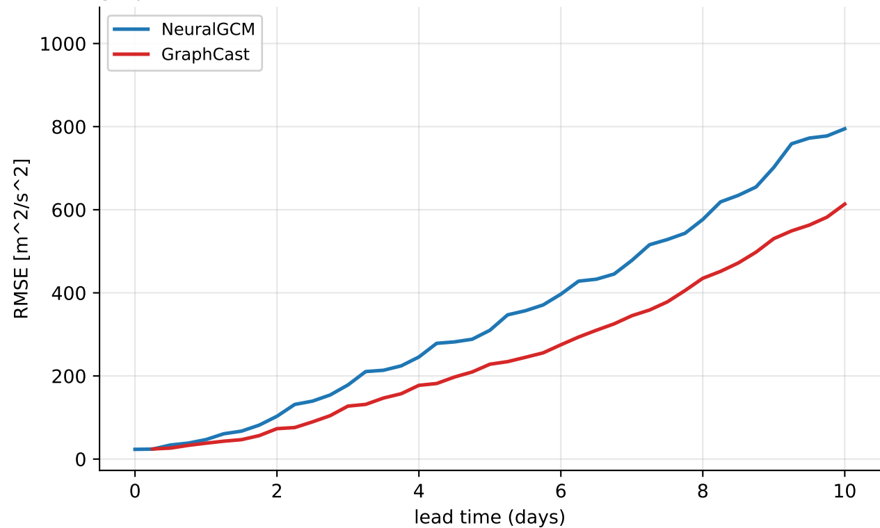
geopotential@500 hPa — mean RMSE over the 3 2026 cordex heat waves (3 events, > p99)
