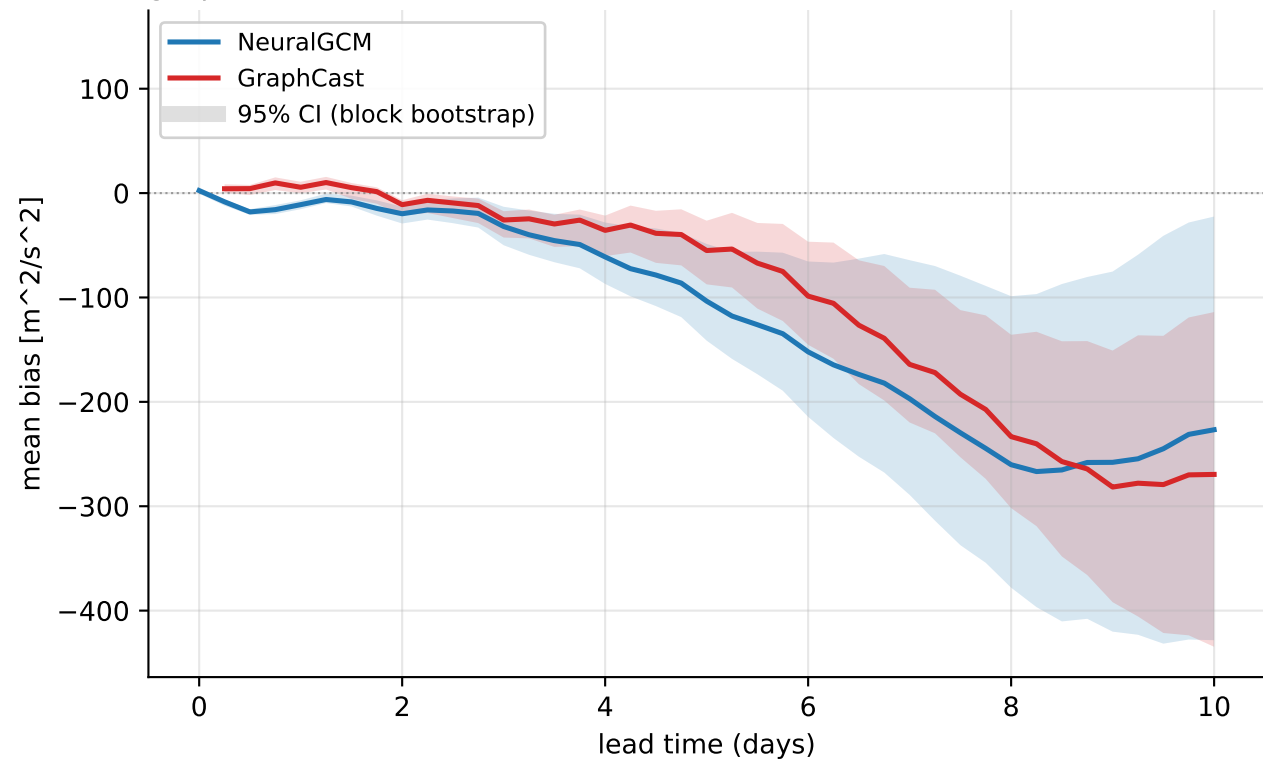
geopotential@500 hPa — mean bias over the 10 2023 mixture heat waves (10 events, > p99)
