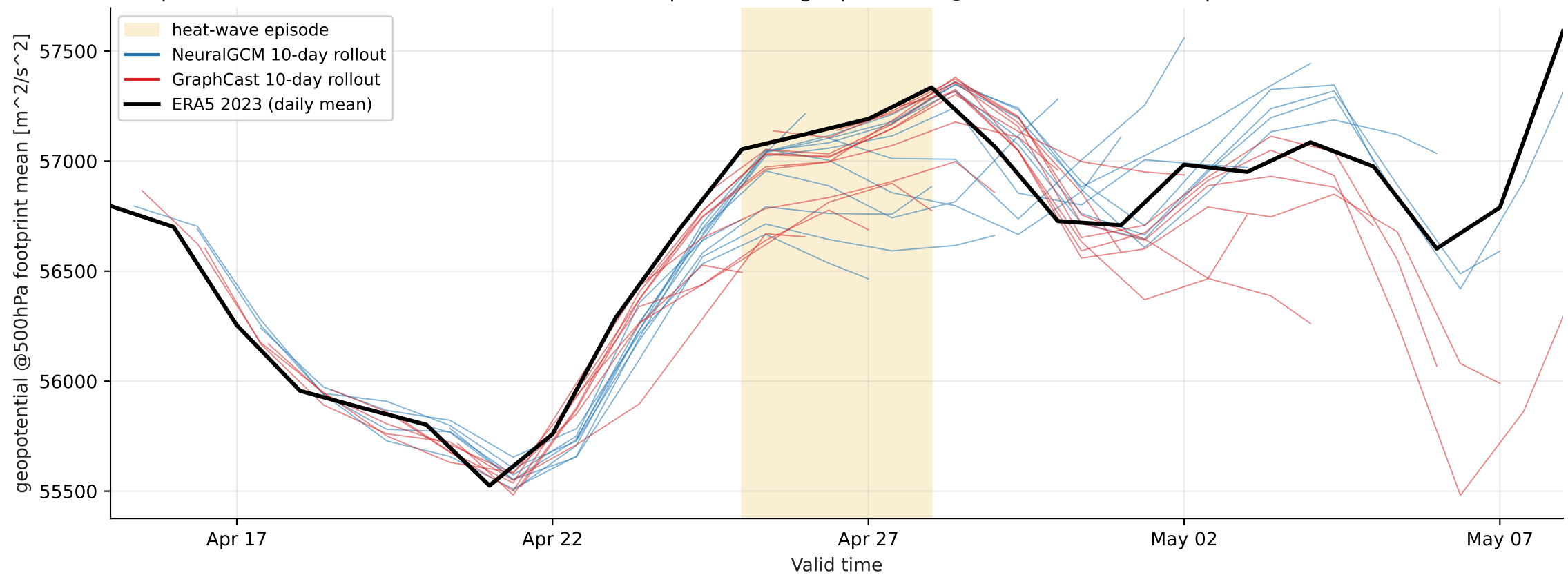
Europe heat-wave 2023-04-25..2023-04-28 — footprint-mean geopotential @ 500 hPa (mixture, > p99)
