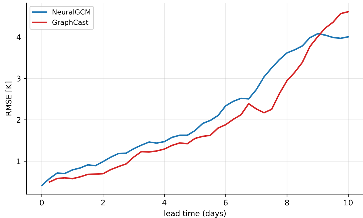
Europe heat-wave 2023-06-10..2023-06-21 — footprint temperature@850 hPa (mean of 22 rollouts)
