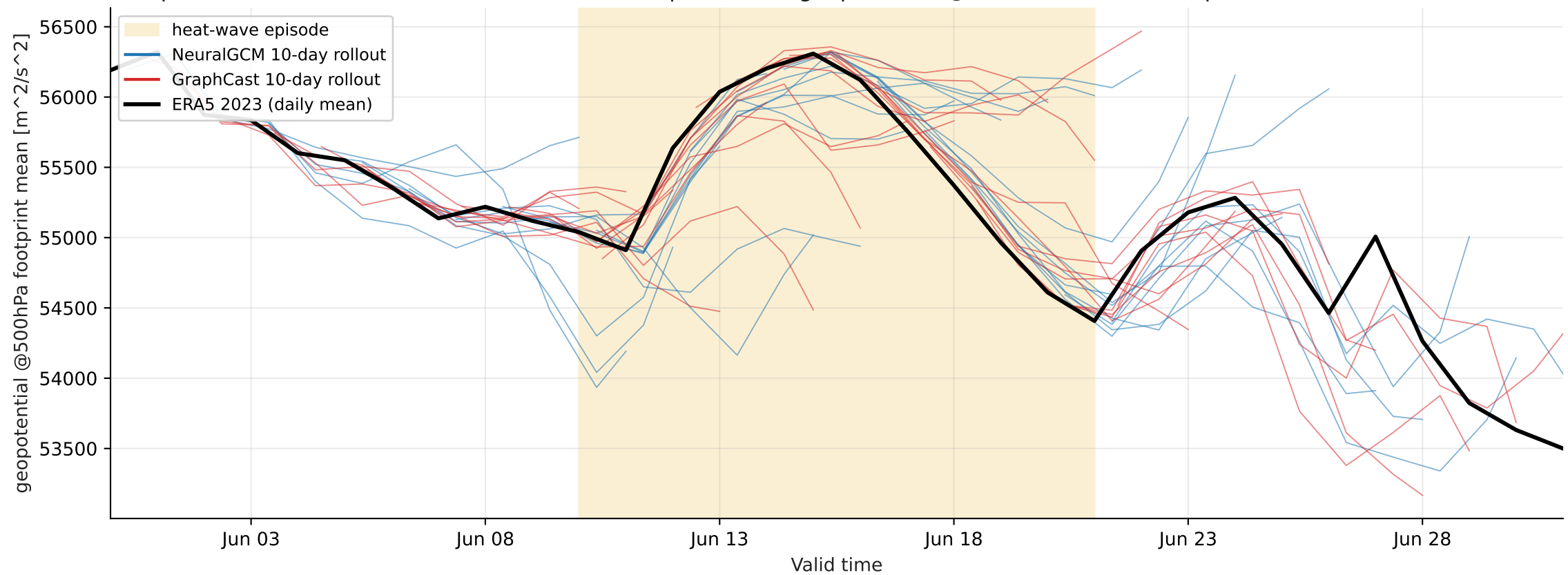
Europe heat-wave 2023-06-10..2023-06-21 — footprint-mean geopotential @ 500 hPa (mixture, > p99)
