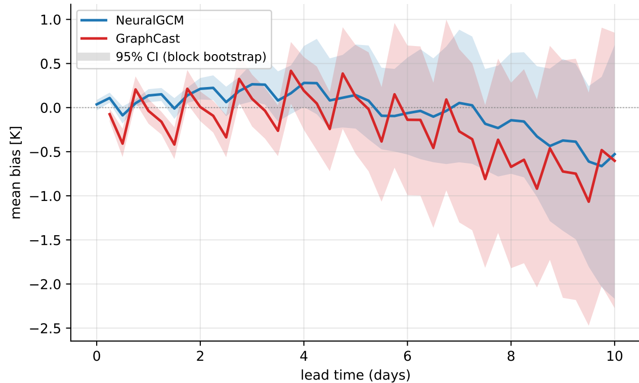
Europe heat-wave 2023-08-08..2023-08-19 — footprint temperature@850 hPa (mean of 22 rollouts)
