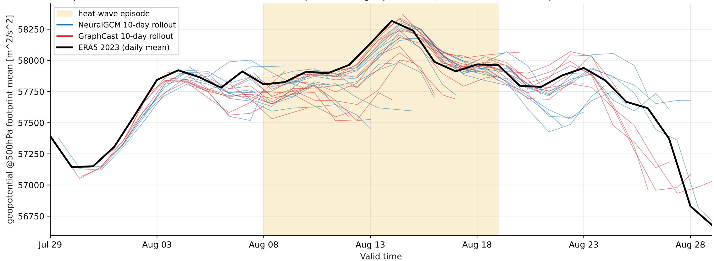
Europe heat-wave 2023-08-08..2023-08-19 — footprint-mean geopotential @ 500 hPa (mixture, > p99)
