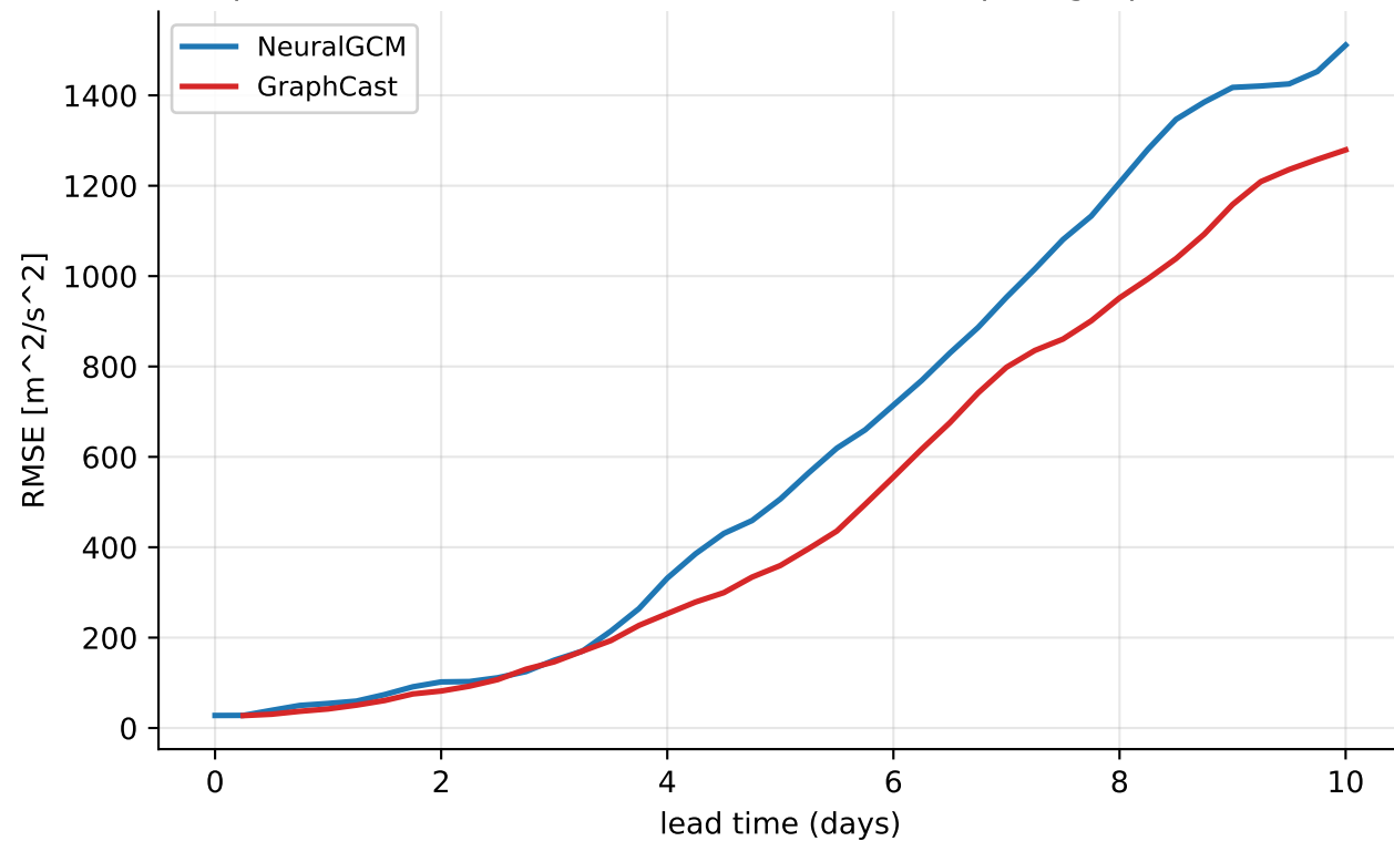
Europe heat-wave 2023-09-04..2023-09-12 — footprint geopotential@500 hPa (mean of 19 rollouts)
