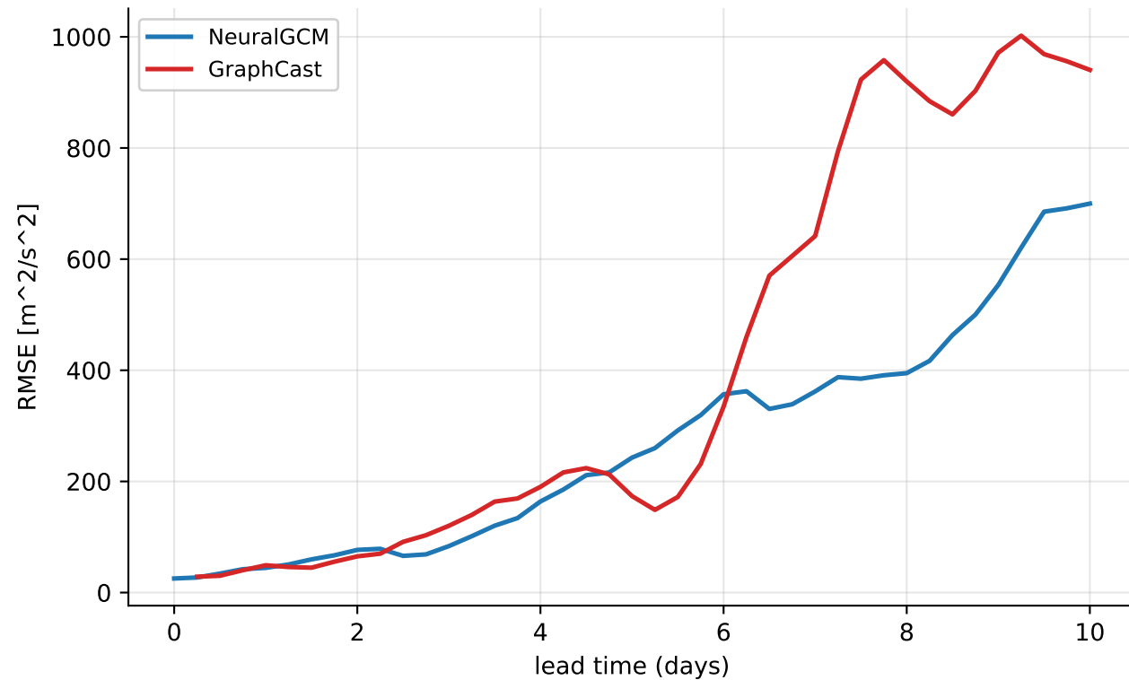
Europe heat-wave 2026-02-21..2026-02-25 — footprint geopotential@500 hPa (mean of 15 rollouts)
