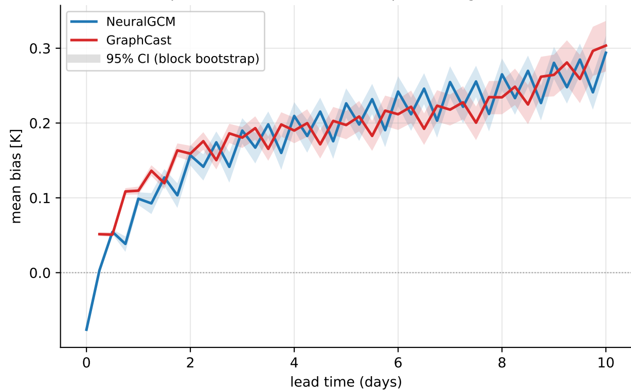
NeuralGCM vs GraphCast — 2049, 850 hPa temperature (global, mean of 221 inits)
