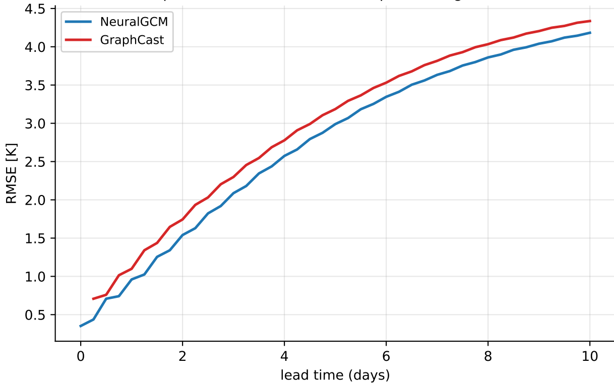
NeuralGCM vs GraphCast — 1955, 850 hPa temperature (global, mean of 355 inits)
