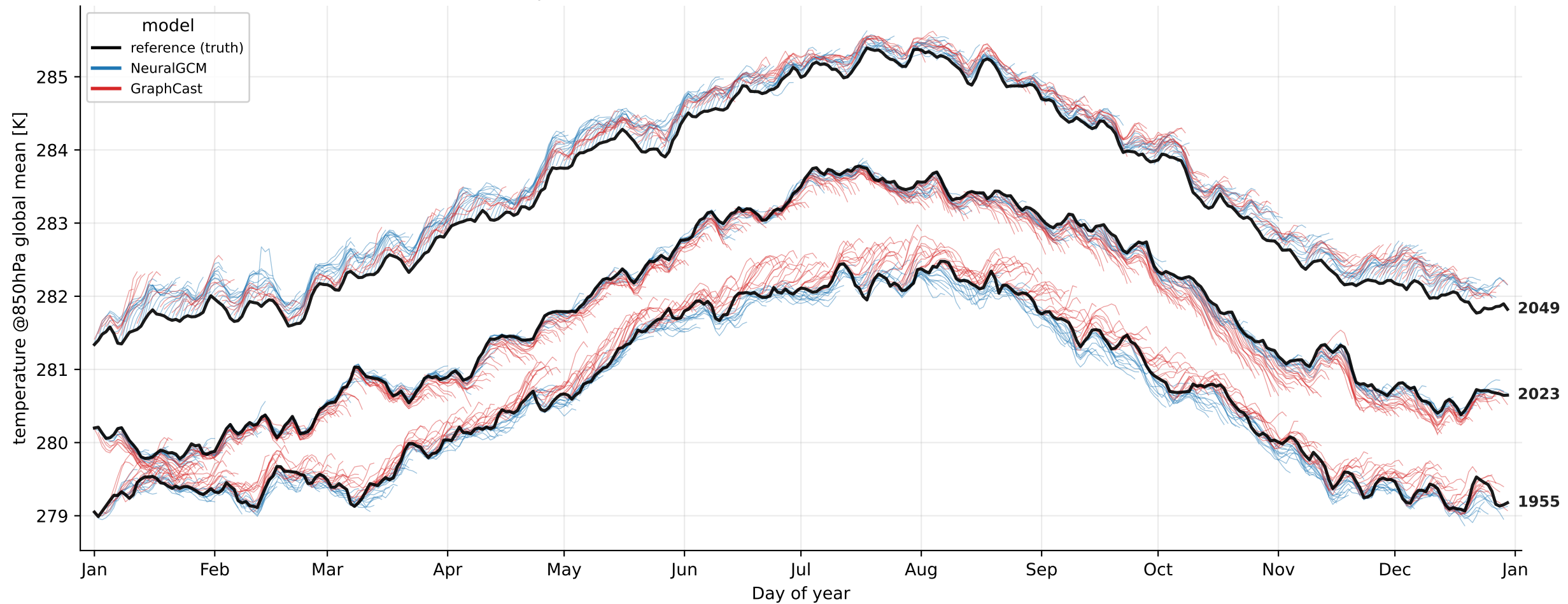
Global-mean temperature at 850 hPa — out-of-distribution rollouts (1955, 2023, 2049)
